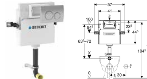
Geberit Delta concealed cistern 12cm, 6/3 litres
